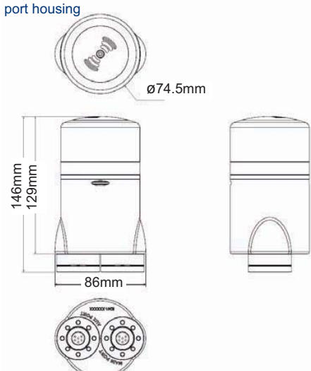
Dual port housing
