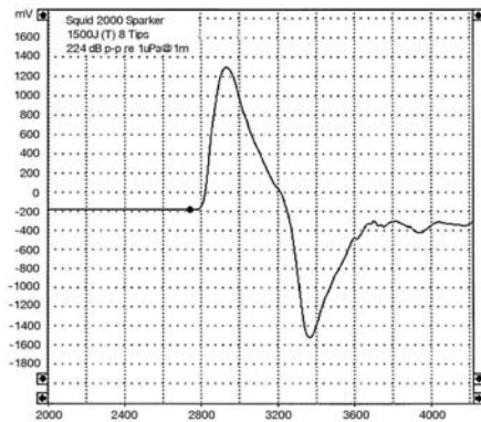
TYPICAL PULSE FROM THE SQUID 2000 AT 1500J
