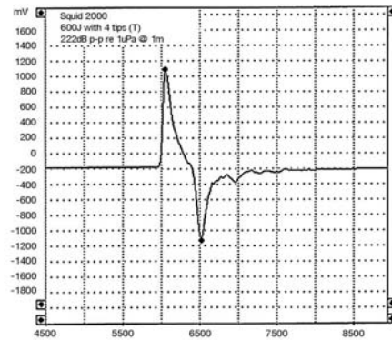
TYPICAL PULSE FROM THE SQUID 2000 AT 600J
