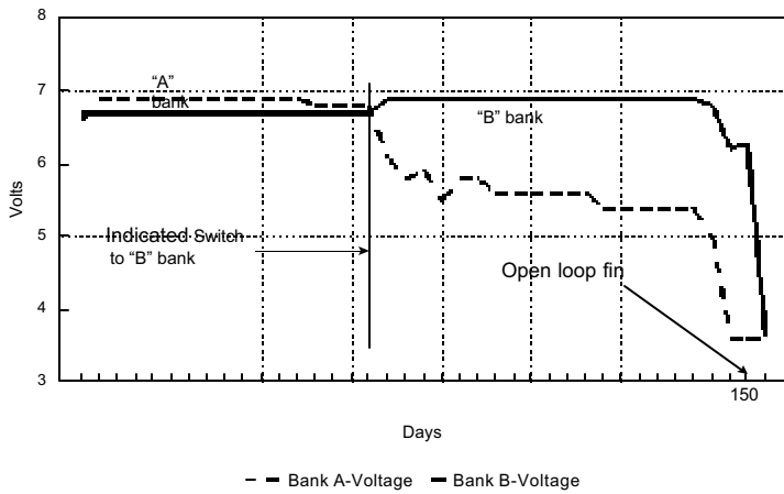
SLB 150 Typical Discharge Characteristics
